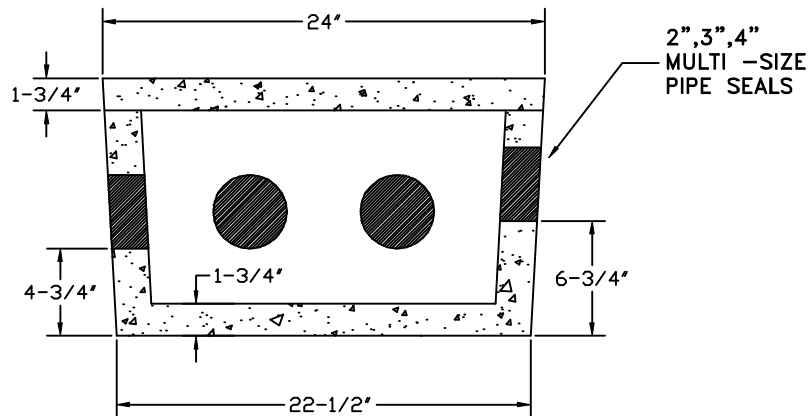
SIDES
