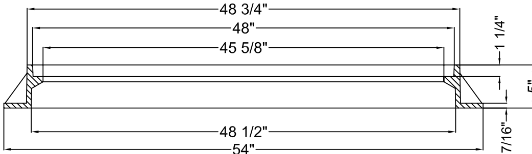
SECTION "B-B"(GRATE)
