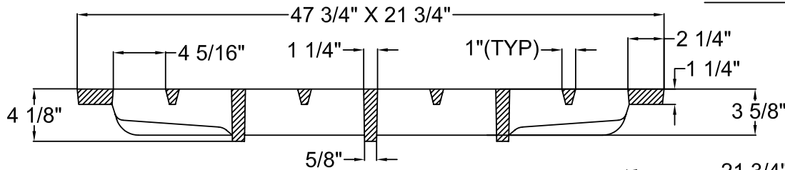
SECTION "A-A"(GRATE)
