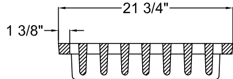
SECTION "B-B"(GRATE)
